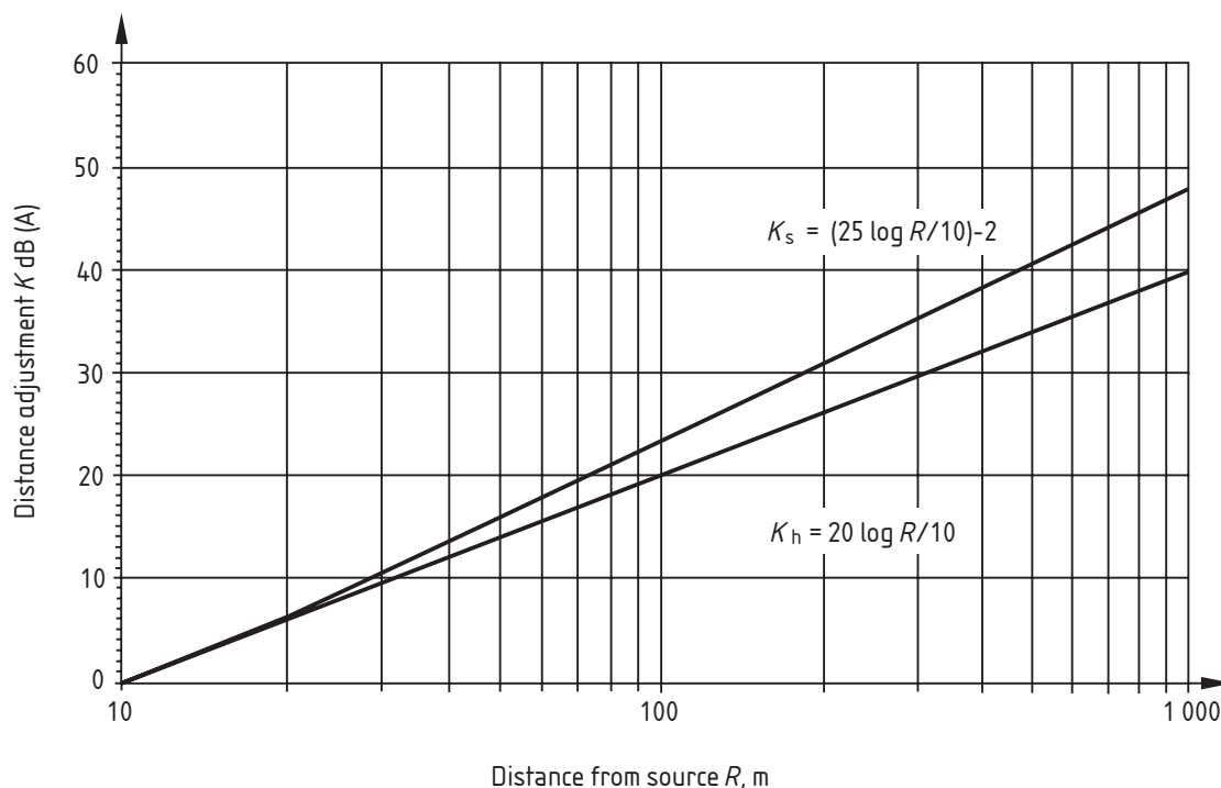
Figure F.2 Distance adjustment K for activity [A_1] L_{Aeq, T} [A_1] method
