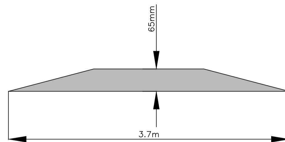
CROSS SECTION VIEW OF SPEED CUSHION
