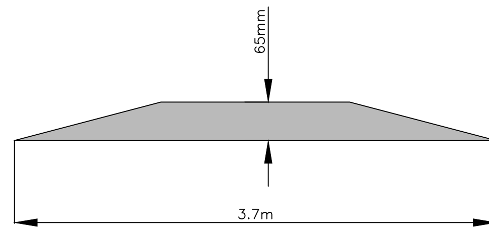
CROSS SECTION VIEW OF SPEED CUSHION
