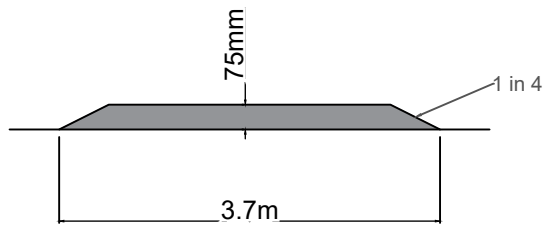
Cross section view of speed cushion
