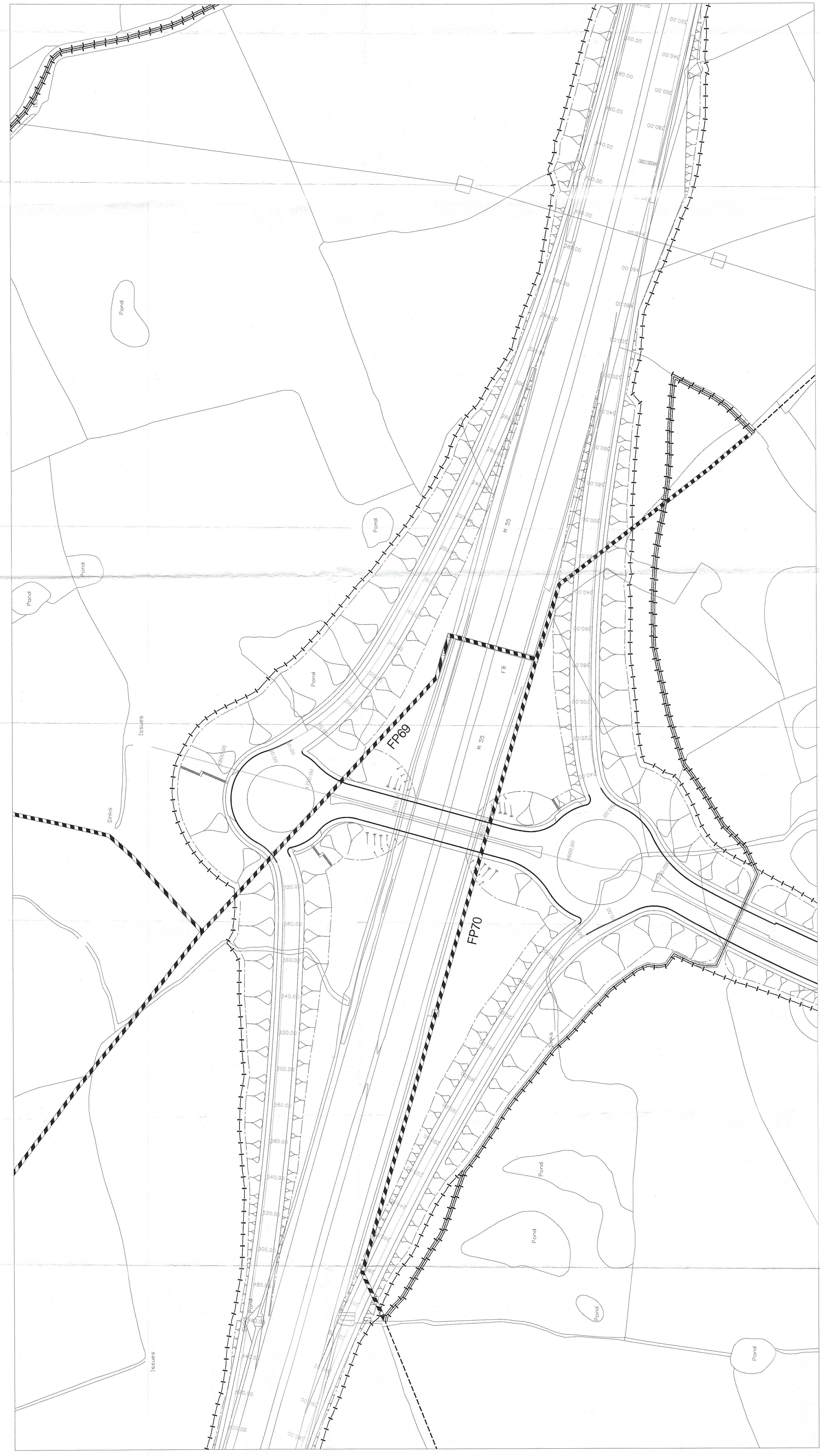
INSET A - WITHOUT I25 SCALE 1:1000
